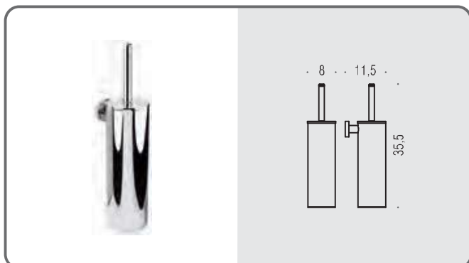
B2707 ○ Porta scopino Hanging brush holder
