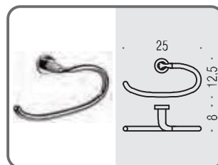
B2731 Porta salvietta ad anello Ring towel holder
